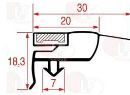
3186767 SNAP-IN GASKET 1007 LENGTH 2000 mm
