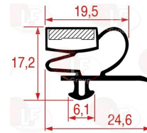
3286097 SNAP-IN GASKET 1011 LENGTH 2000 mm
