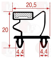
3186877 SNAP-IN GASKET 1010 LENGTH 2000 mm
