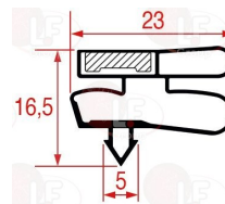
3286128 SNAP-IN GASKET 1014 LENGTH 2000 mm
