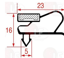
3286126 SNAP-IN GASKET 1012 LENGTH 2000 mm
