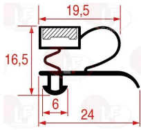
3286124 SNAP-IN GASKET 1006 LENGTH 2000 mm
