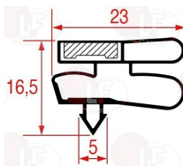
3286127 SNAP-IN GASKET 1013 LENGTH 2000 mm
