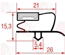
3286063 SNAP-IN GASKET 1016 LENGTH 2000 mm
