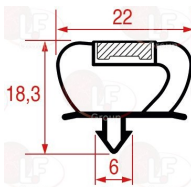
3286162 SNAP-IN GASKET 1012 - 2000 mm
