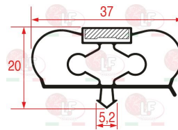
3286096 SNAP-IN GASKET 1017 LENGTH 2500 mm
