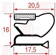
3186874 SNAP-IN GASKET 1001 LENGTH 2000 mm
