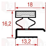
3286141 MIDDLE EDGED GASKET 2007 LENGTH 2000 mm
