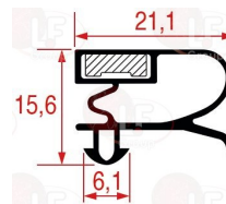
3286096 SNAP-IN GASKET 1017 LENGTH 2500 mm
