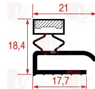
3186867 MIDDLE EDGED GASKET 2005 LENGTH 2000 mm
