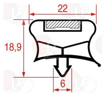
3286063 SNAP-IN GASKET 1016 LENGTH 2000 mm
