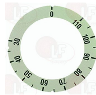
3241457 SELF-STICK DISK 30-110°C external \varnothing 63 mm
